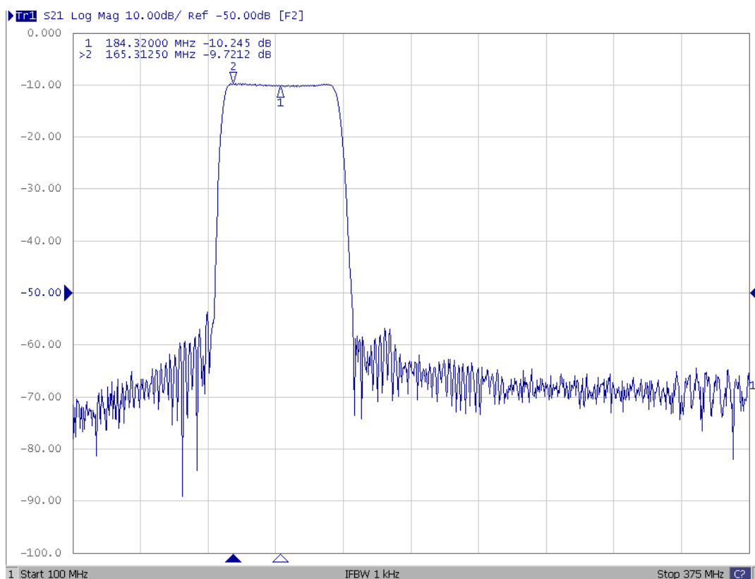
Fig4. Horizontal: 27.5MHz/Div Vertical: 10dB/Div
