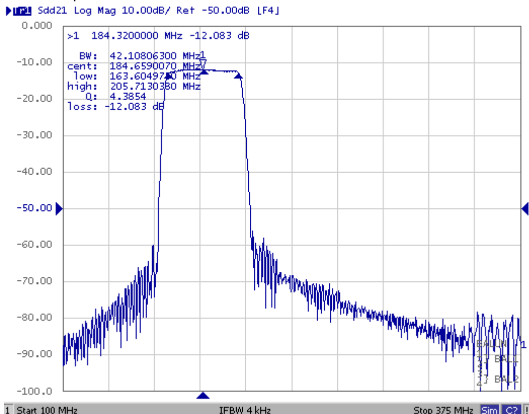
Fig1. Horizontal: 30MHz/Div Vertical: 10dB/Div
