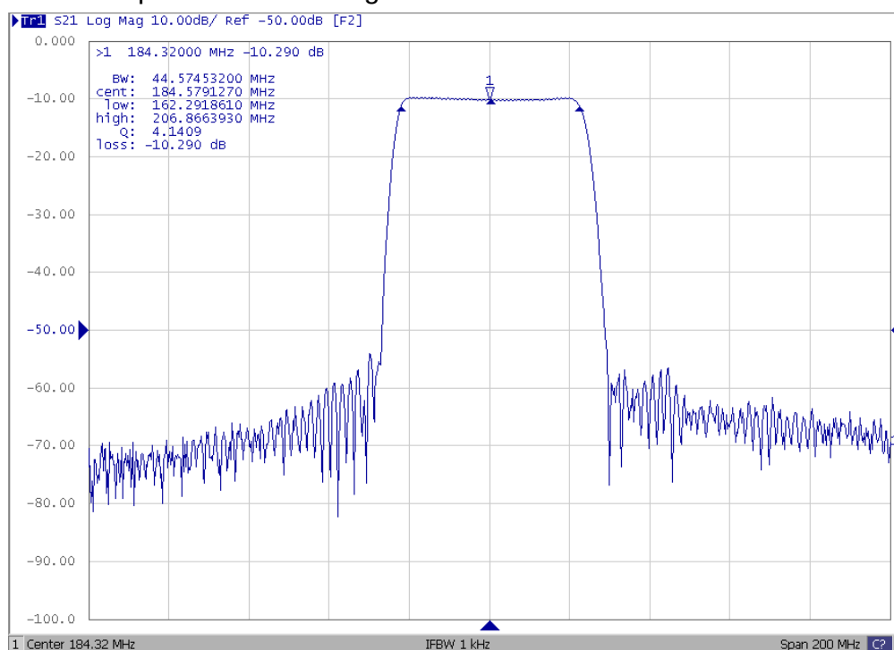
Fig1. Horizontal: 20MHz/Div Vertical: 10dB/Div
