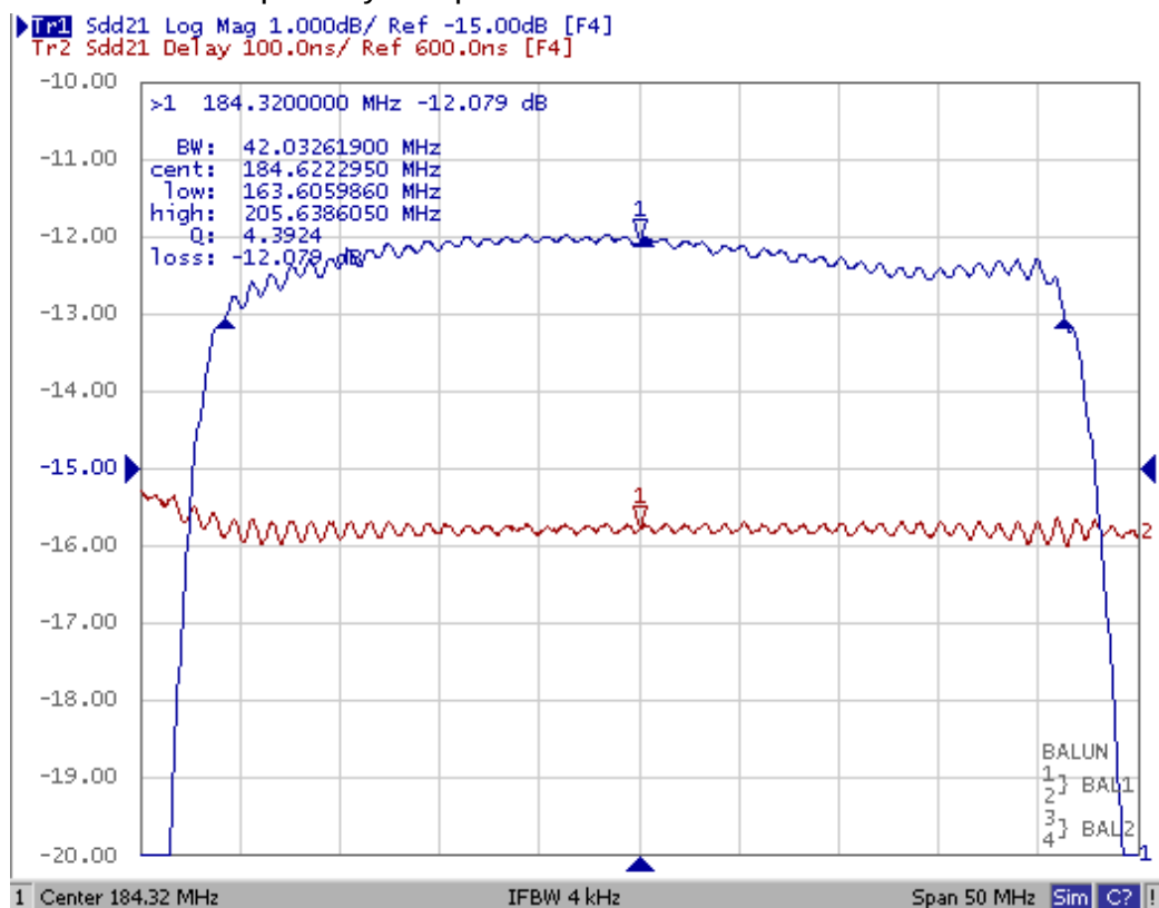
Fig2. Horizontal: 5MHz/Div Vertical: 1dB/Div Vertical: 100ns/Div
